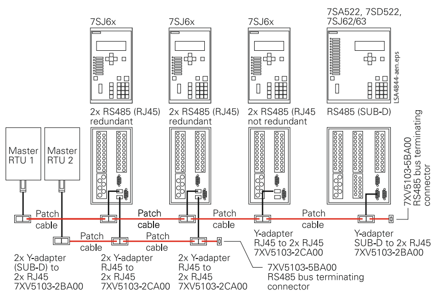
Fig. 13/6 Connection of SIPROTEC 4 to a (redundant) control system
