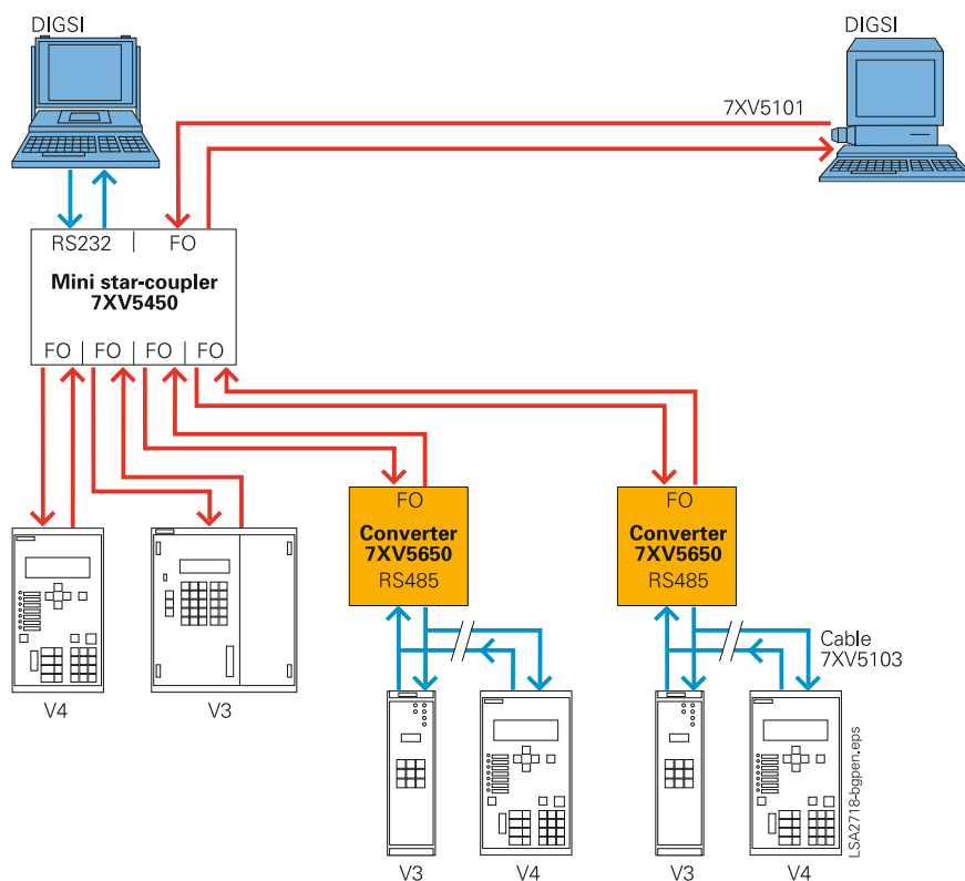
Fig. 13/29 Optical star structure with connected RS485 interfaces
