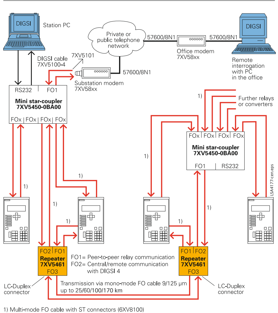
Fig. 13/19 Transfer of protection data and remote control of a substation via an optical long-distance connection
