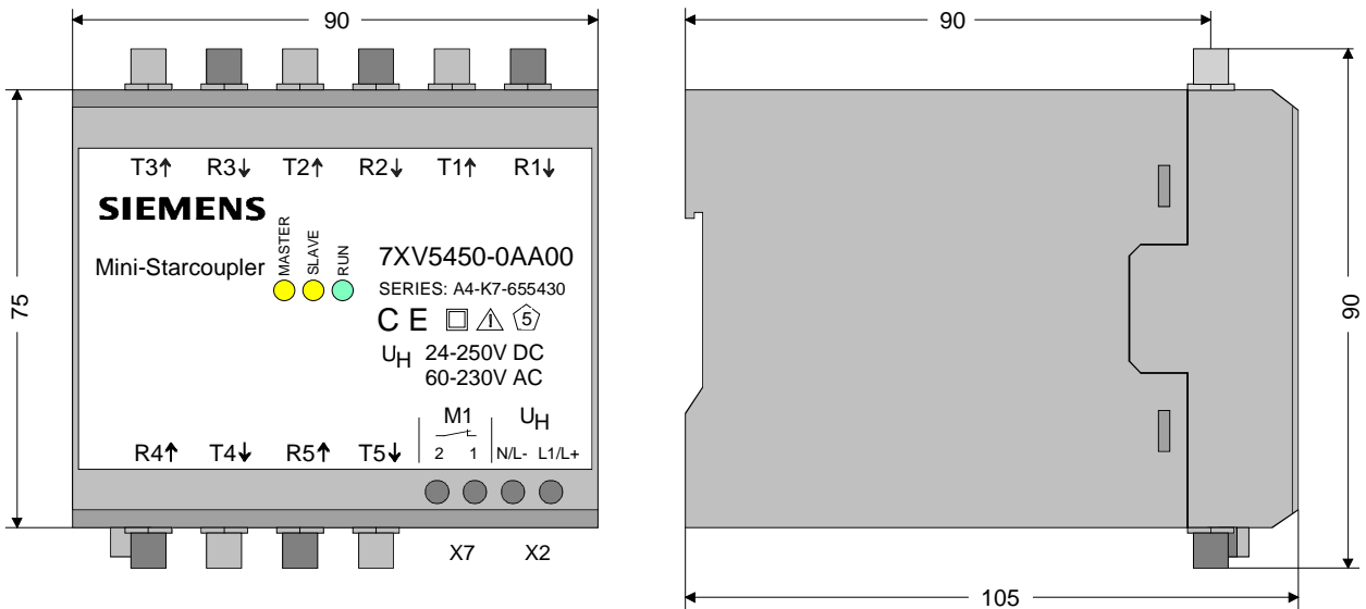
Fig. 1: Dimension Drawings
