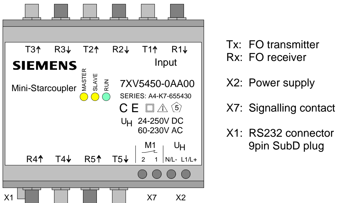
Fig. 2: Terminal Assignment
