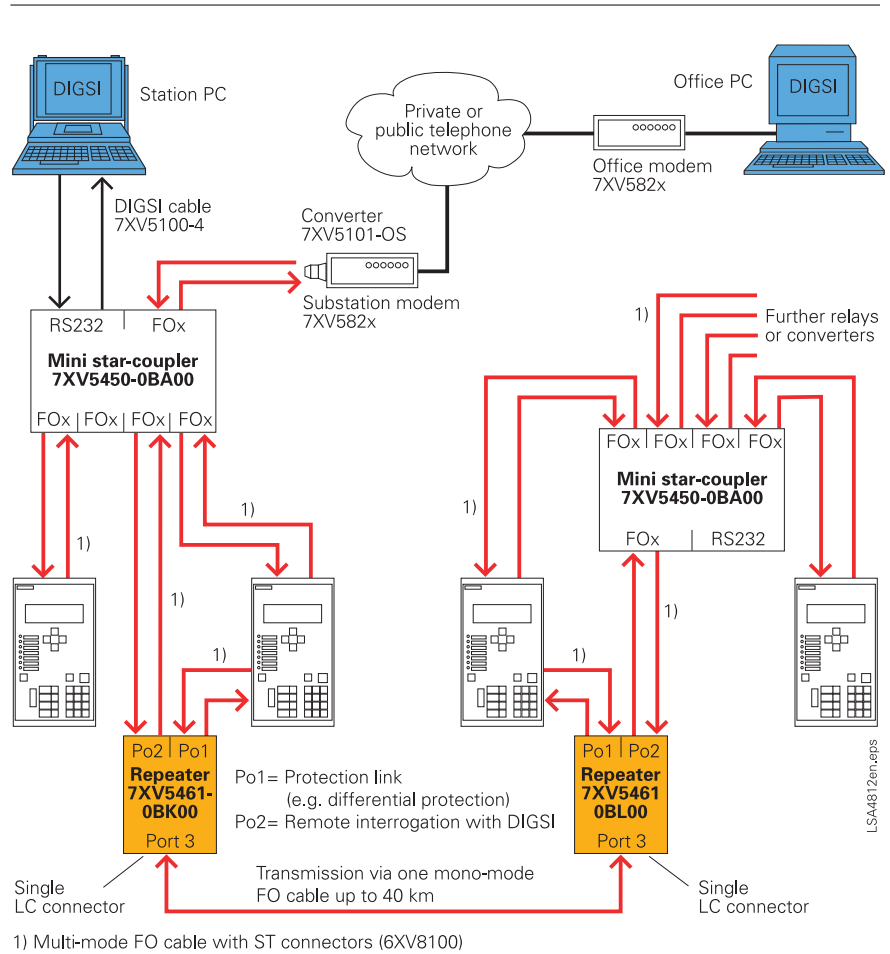
Fig. 13/21 Transfer of protection data signals and remote control/integration via one mono-mode FO cable (Note: Devices 7XV5461-0BK00 and 7XV5461-0BL00 must be used in pairs)
