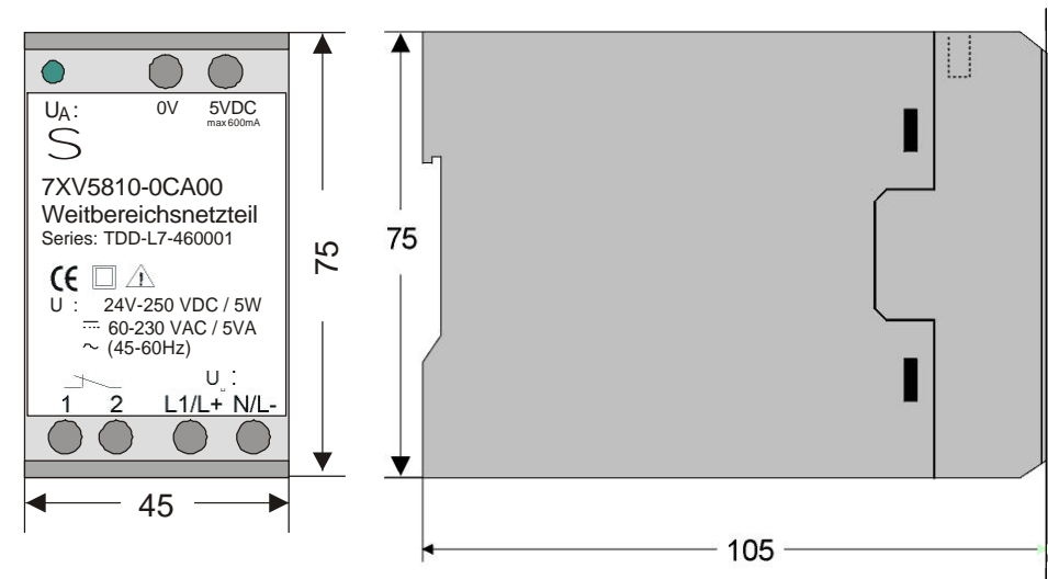
Abb. 4: Dimension Drawings
