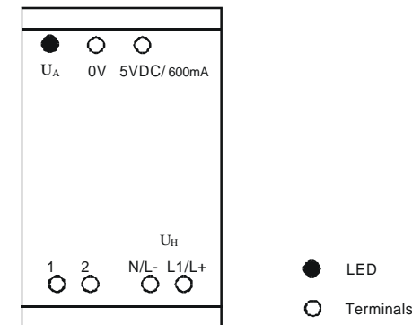
Fig. 2: Position and assignment of the terminals
