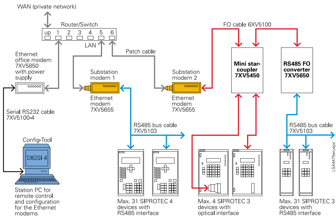
Fig. 15/72 Operation of various SIPROTEC protection unit generations via Ethernet modems
