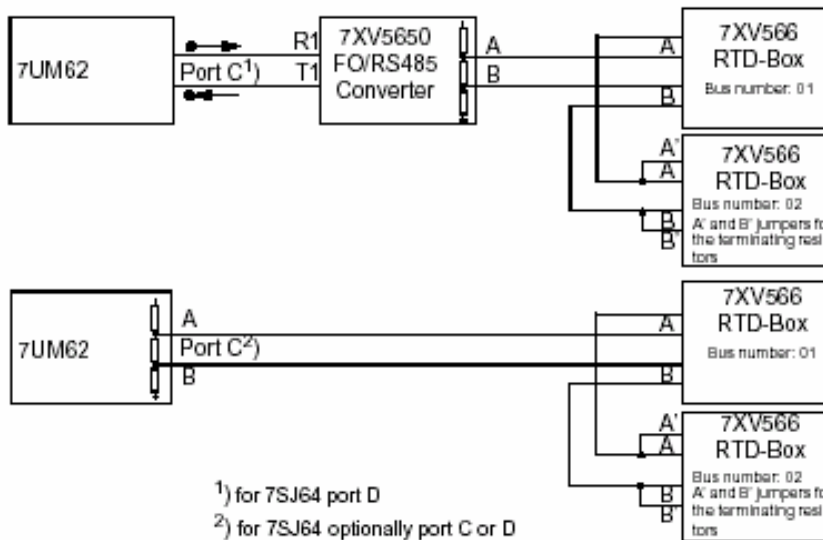
Figure A-42 Half-duplex operation with two RTD-Boxes above: optical design (2 FOs); below: design with RS485
