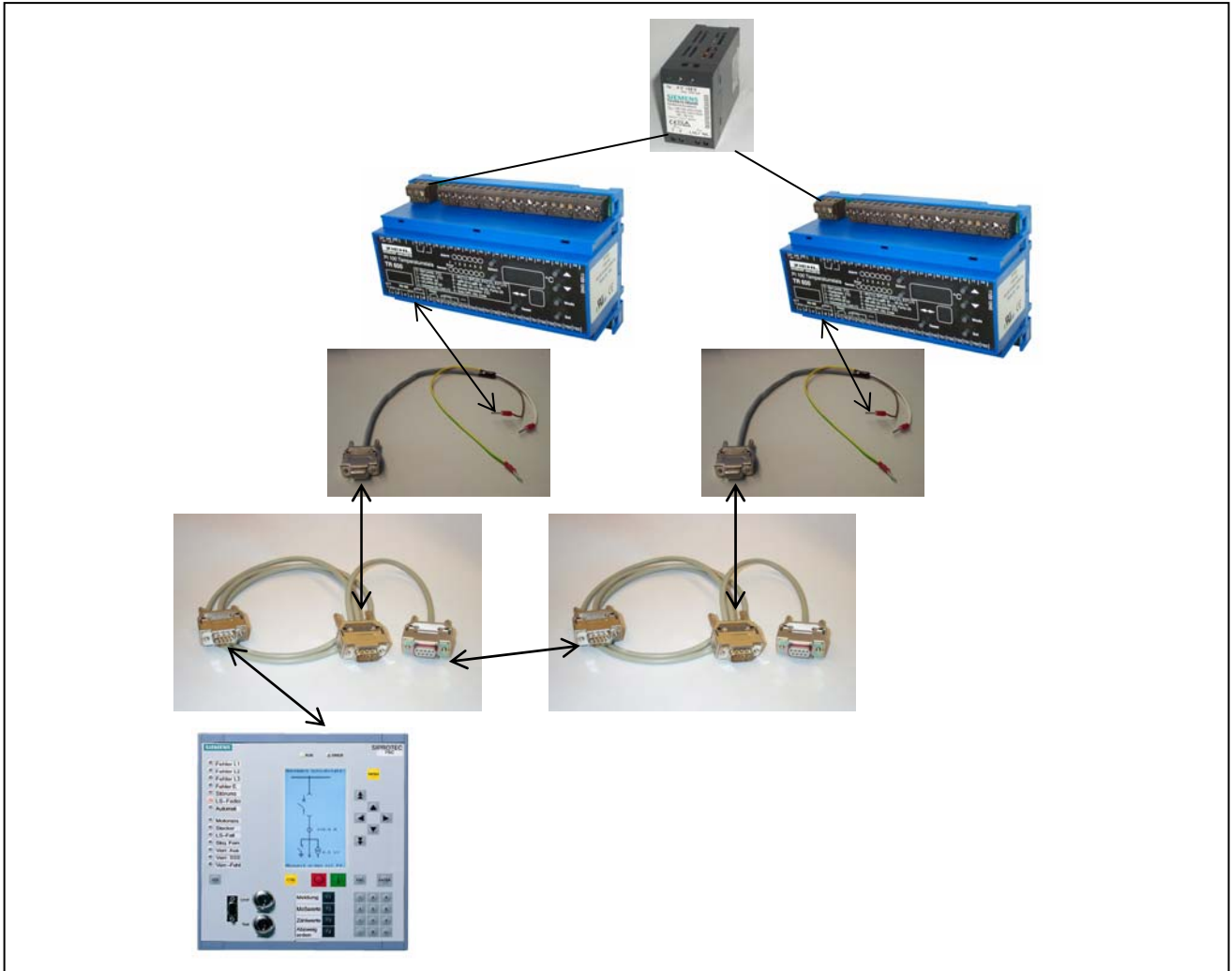
Picture 11: Connection with 2 RTD boxes
