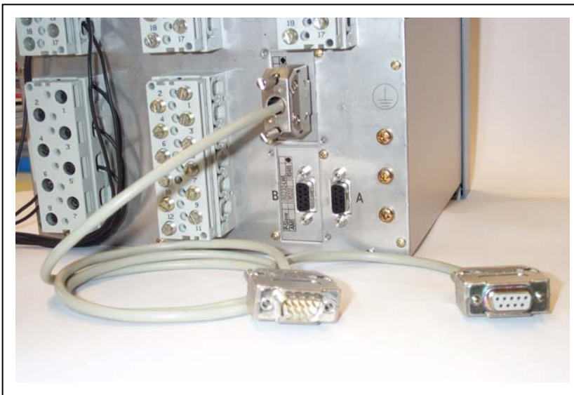
Picture 2: Connection to service port at rear side (port C )
