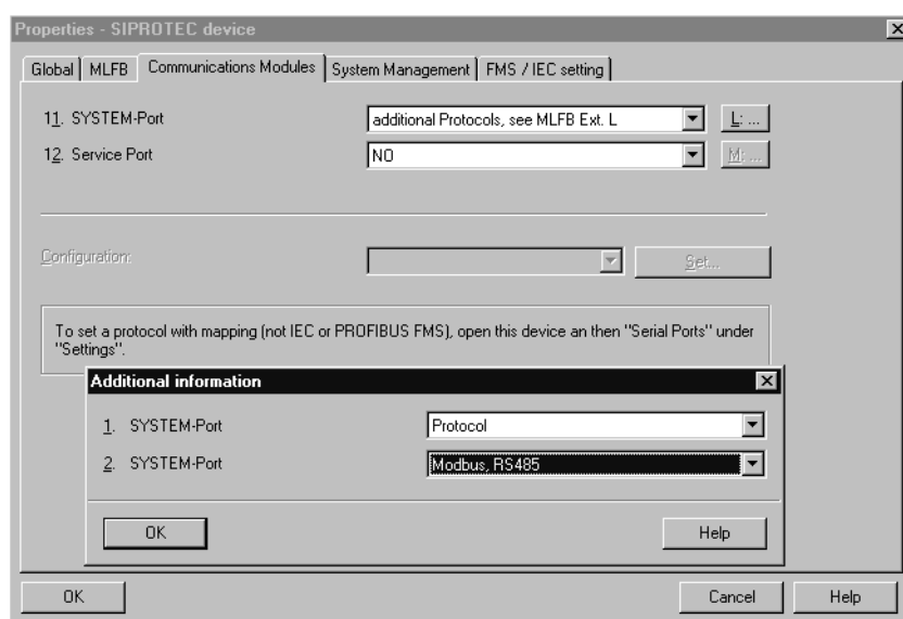
Figure 4-3 DIGSI 4.3: Modbus protocol assignment
