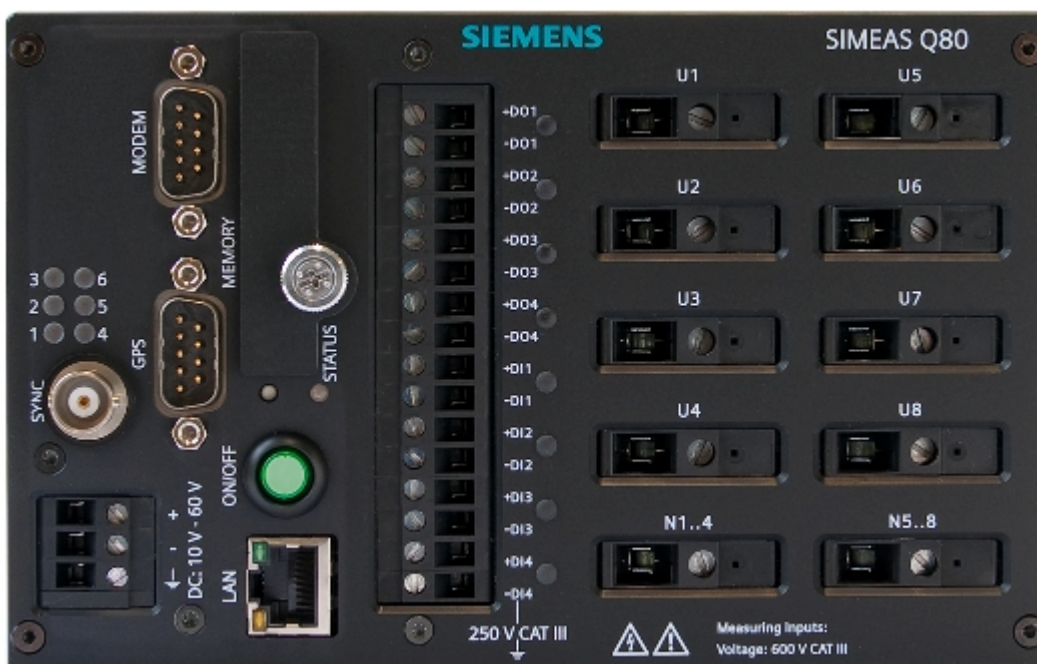
SIMEAS Q80 7KG8080 - 1 with 8 voltage inputs
