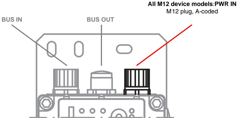
Figure 4.6: Location and designation of the M12 connections
