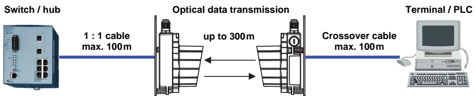
Figure 10.4: Network expansion
