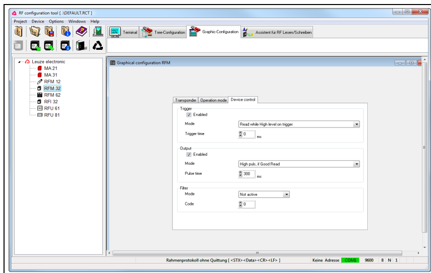
Figura 7.4: RF-Config – Ficha Device control
