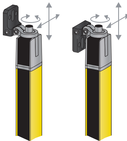
Figure 6.8: Mounting via BT-R swivel mount
