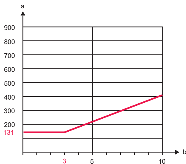
Figure 6.3: Minimum distance to reflective surfaces depending on protective field width
