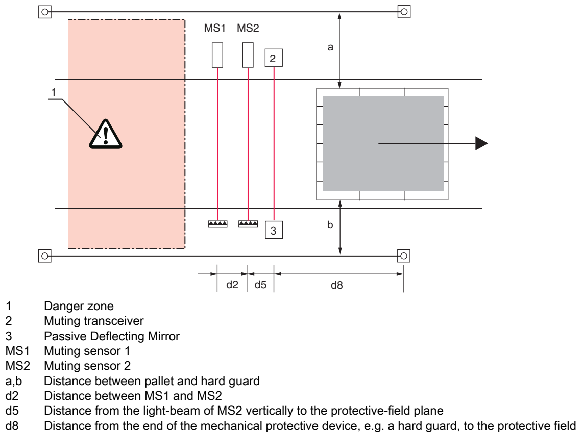
Figure 6.10: Typical arrangement of the muting sensors for sequence controlled 2-sensor muting (example acc. to IEC TS 62046)
