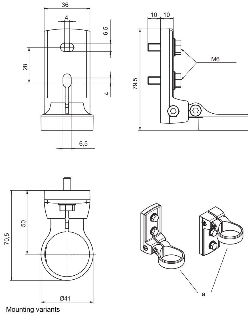
Figure 14.10: Swivel mount BT-240C
