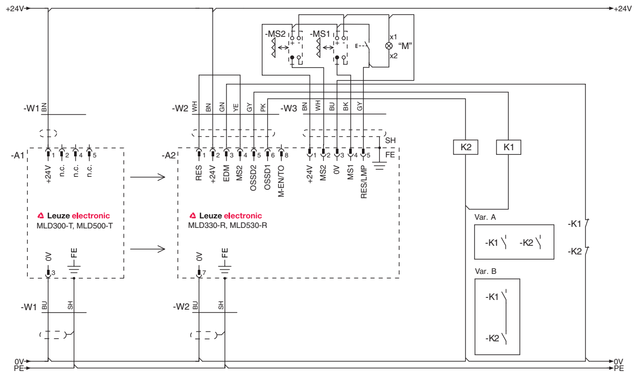
Figure 7.11: Connection example MLD 330, MLD 530 (transmitter-receiver system): timing controlled 2-sensor muting with muting timeout 10 min (transceiver connected in an analogous manner)
