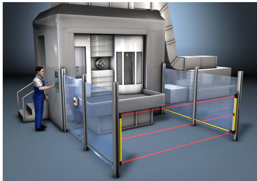
Figure 5.6: Access guarding based on AS-i safety at work with MLD 500/AS-i at a machining center
