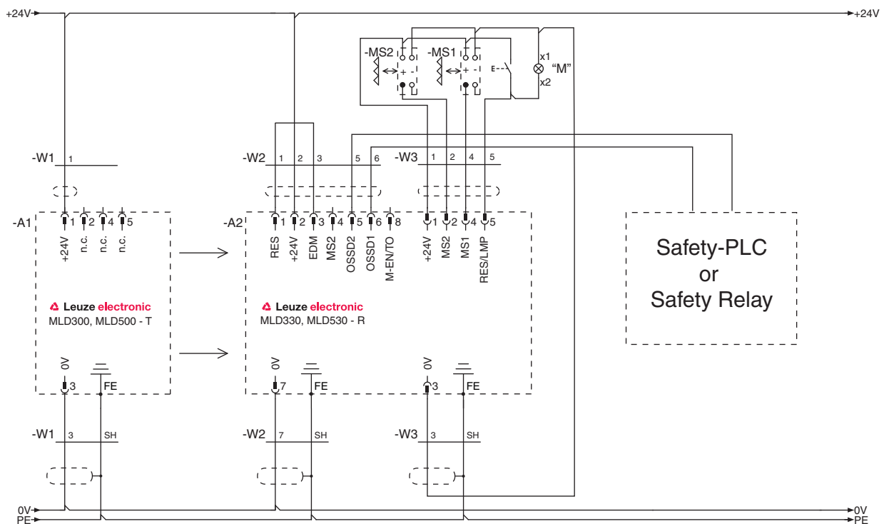
Figure 7.16: Connection example MLD 330, MLD 530 (transmitter-receiver system): sequence controlled 2-sensor muting with muting timeout 8 h (transceiver connected in an analogous manner)
