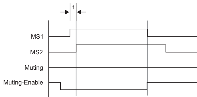
Figure 4.10: No valid muting-enable signal
