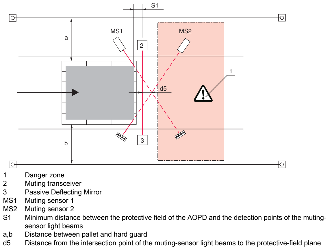
Figure 6.8: Typical arrangement of the muting sensors for timing controlled 2-sensor muting (example acc. to IEC TS 62046)
