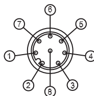
Figure 7.3: Pin assignment receiver MLD 320, MLD 520
