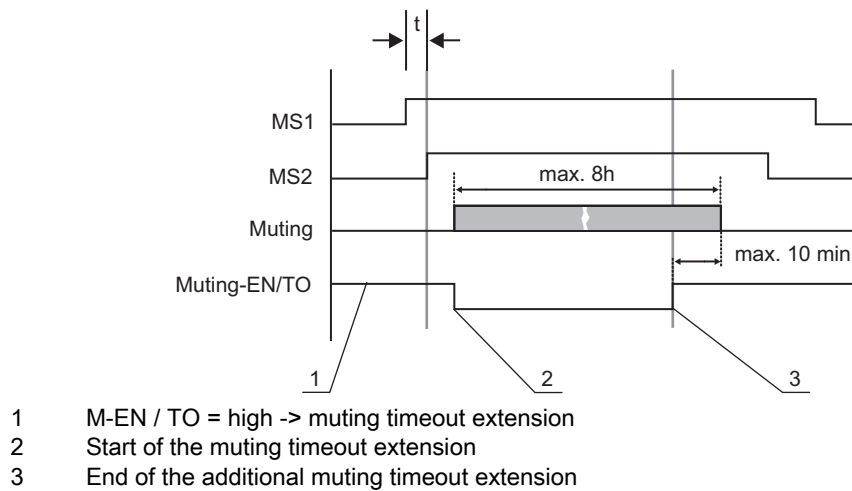
Figure 4.6: Muting timeout extension
