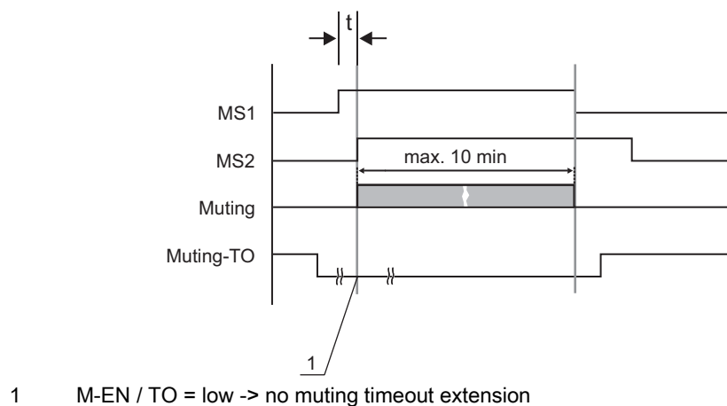
Figure 4.7: No valid signal for timeout extension
