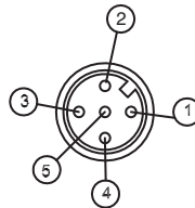
Figure 7.7: MLD 500/AS-i pin assignment (transmitter, receiver/transceiver, connection socket for external muting indicator)
