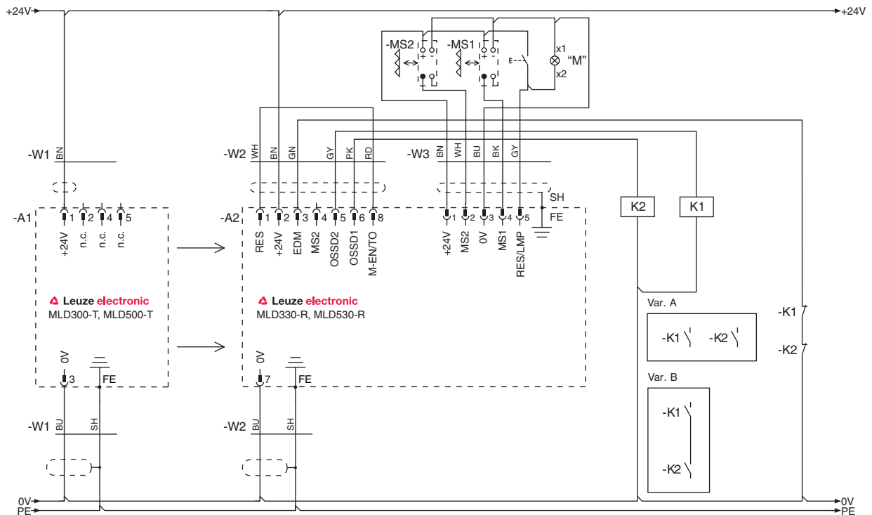
Figure 7.13: Connection example MLD 330, MLD 530 (transmitter-receiver system): timing controlled 2-sensor muting with muting timeout 8 h (transceiver connected in an analogous manner)
