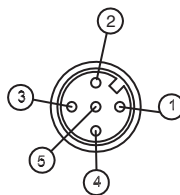
Figure 7.1: Pin assignment transmitter MLD 300, MLD 500
