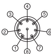
Figure 7.5: Assignment 5-pin socket - receiver MLD 330, MLD 530
