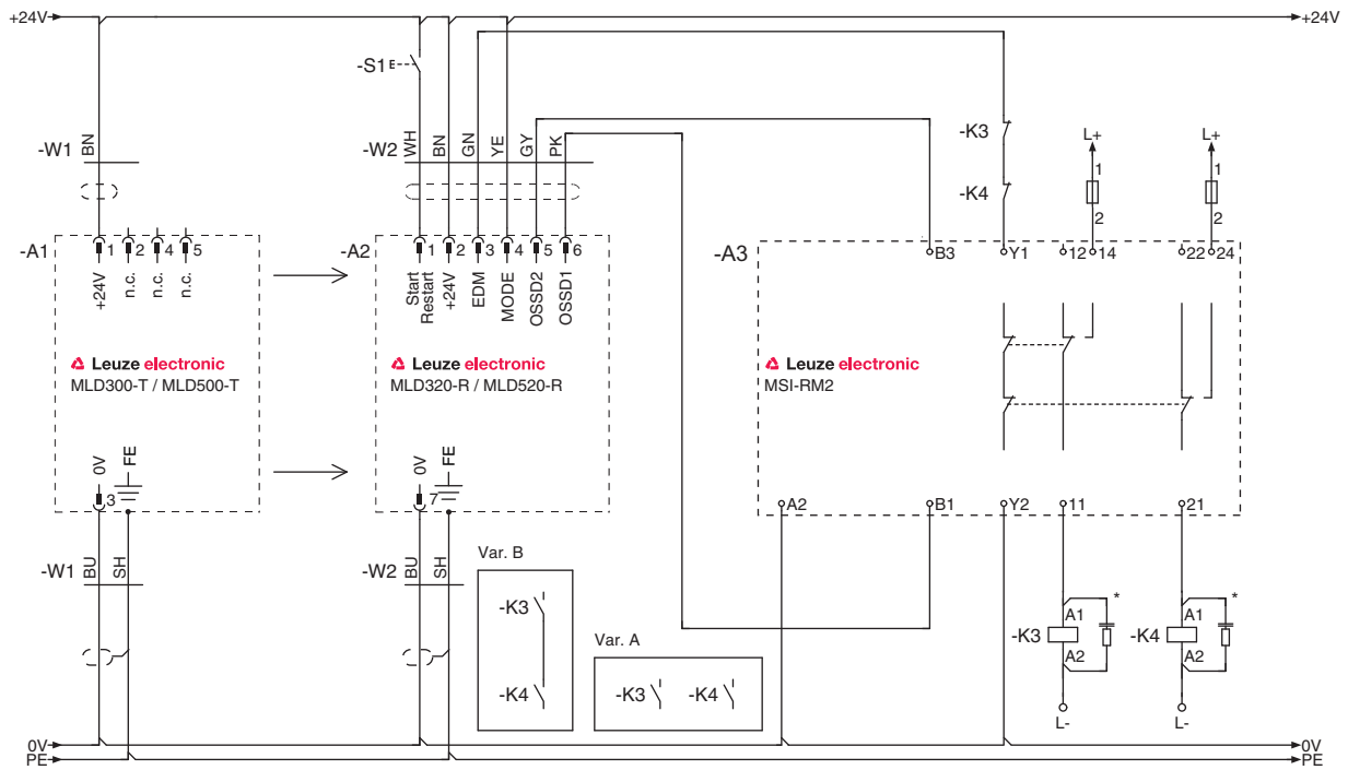
Figure 7.10: Connection example MLD 320, MLD 520 (transmitter-receiver system) and MSI-RM2, with EDM and RES (transceiver connected in an analogous manner)
