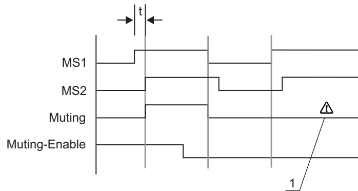
Figure 4.11: Example: Fault at the muting-enable cable
